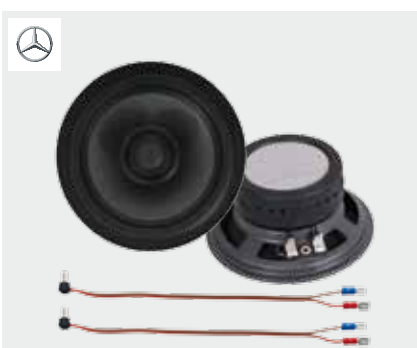
IL-X4.7 MB W124 Front 4.75 inch (12 cm) Coaxial Set 20 mm Silk dome Tweeter Max. 80 Watts Minimum Amplifier Power: 30 Watts Frequency Responce: 65 Hz - 21 kHz Part.-No.: 231240 UVP: 99,00 €
