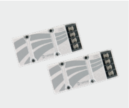
Passiv Crossover Lowpass For additional midbass 270 Hz - 12 dB - 4 Ω
