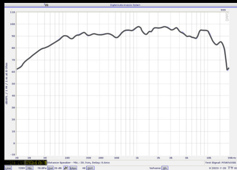
E5PRO6MPR MIDRANGE FREQUENCY RESPONSE
