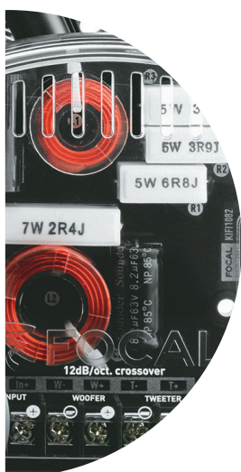
Adjustable tweeter level
